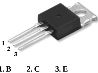
TO-220AB
